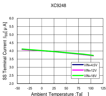
(15) SS Terminal Current vs. Ambient Temperature
