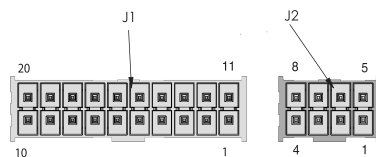
AC Connector
