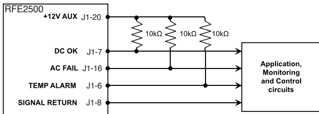
Fig-1.9 Open collector signals are shunted by internal 24V zeners
