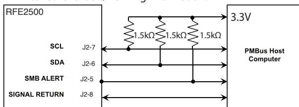
Fig-3.6 PMBus Typical connection
