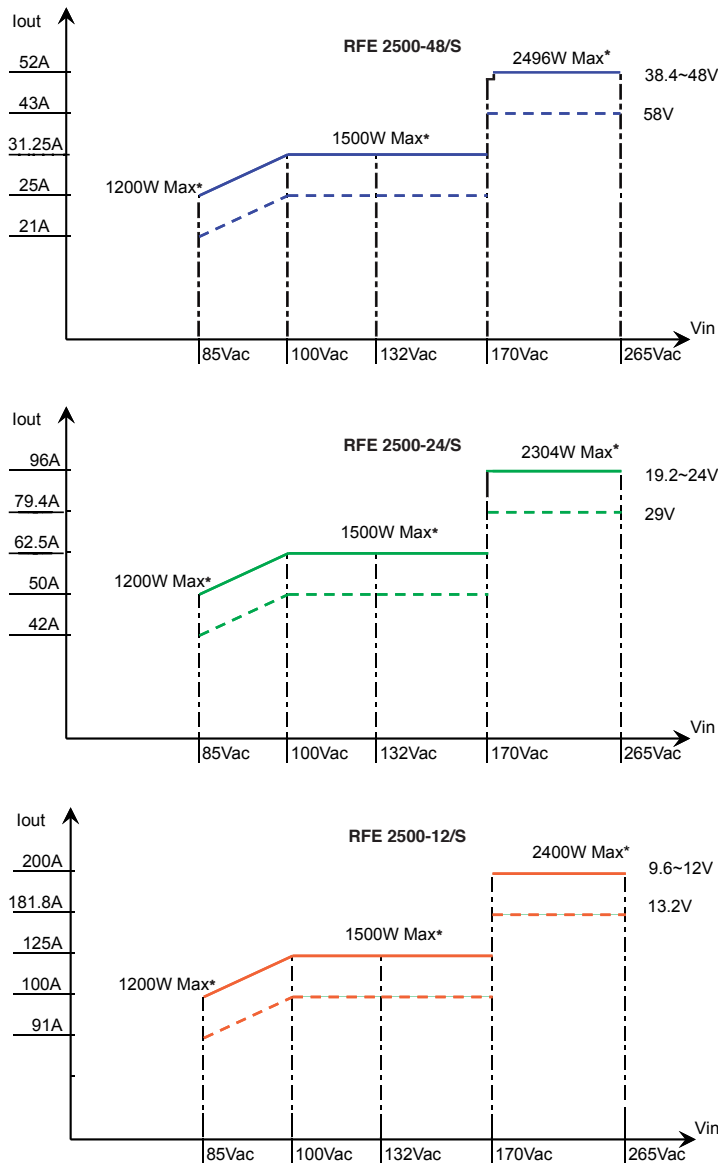
Fig-1 RFE2500 rated output Current and Voltage versus Line Voltage.
