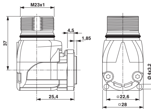
Dimensioned drawing
