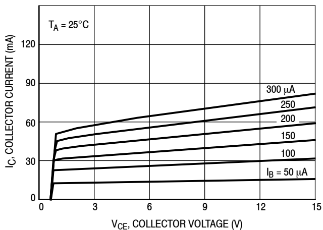
Figure 2. I_C - V_{CE}
