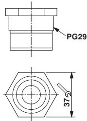
Dimensional drawing
