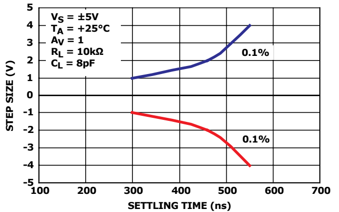
FIGURE 26. STEP SIZE vs SETTling TIME
