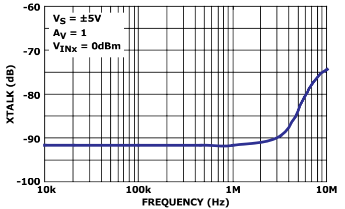
FIGURE 24. CHANNEL SEPARATION vs FREQUENCY RESPONSE
