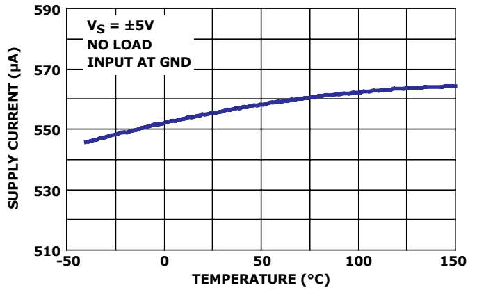
FIGURE 12. SUPPLY CURRENT PER AMPLIFIER vs TEMPERATURE
