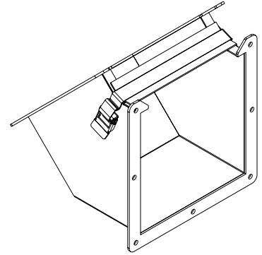
ISOMETRIV VIEW
