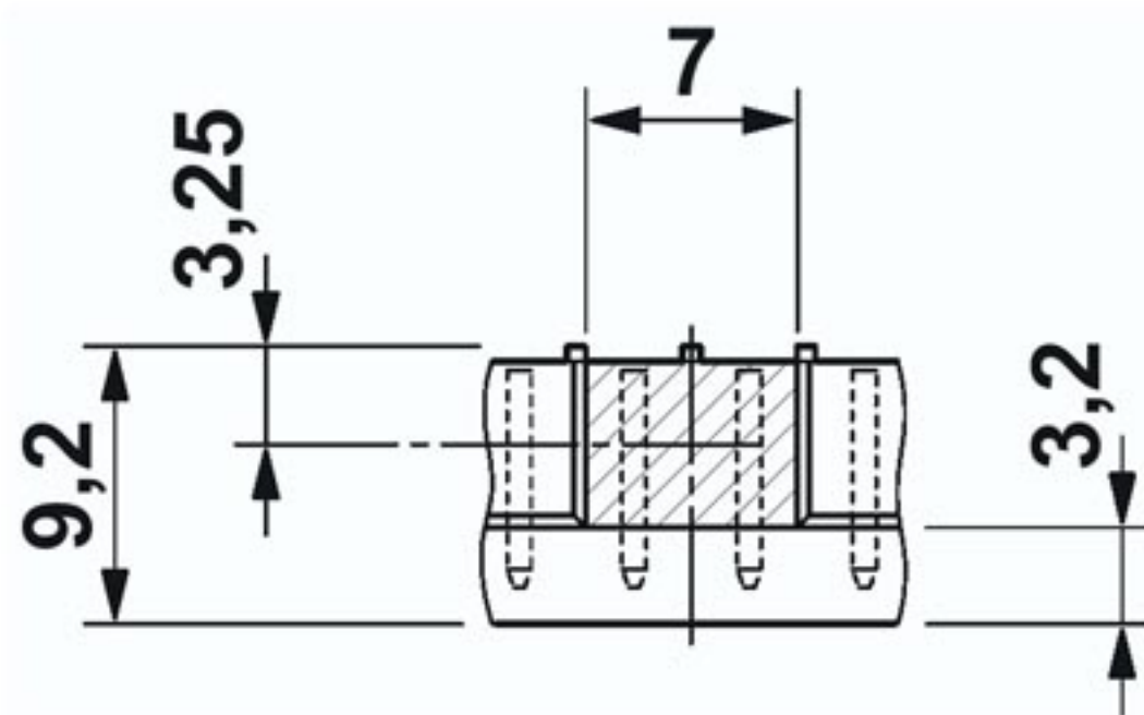
Dimensioned drawing
