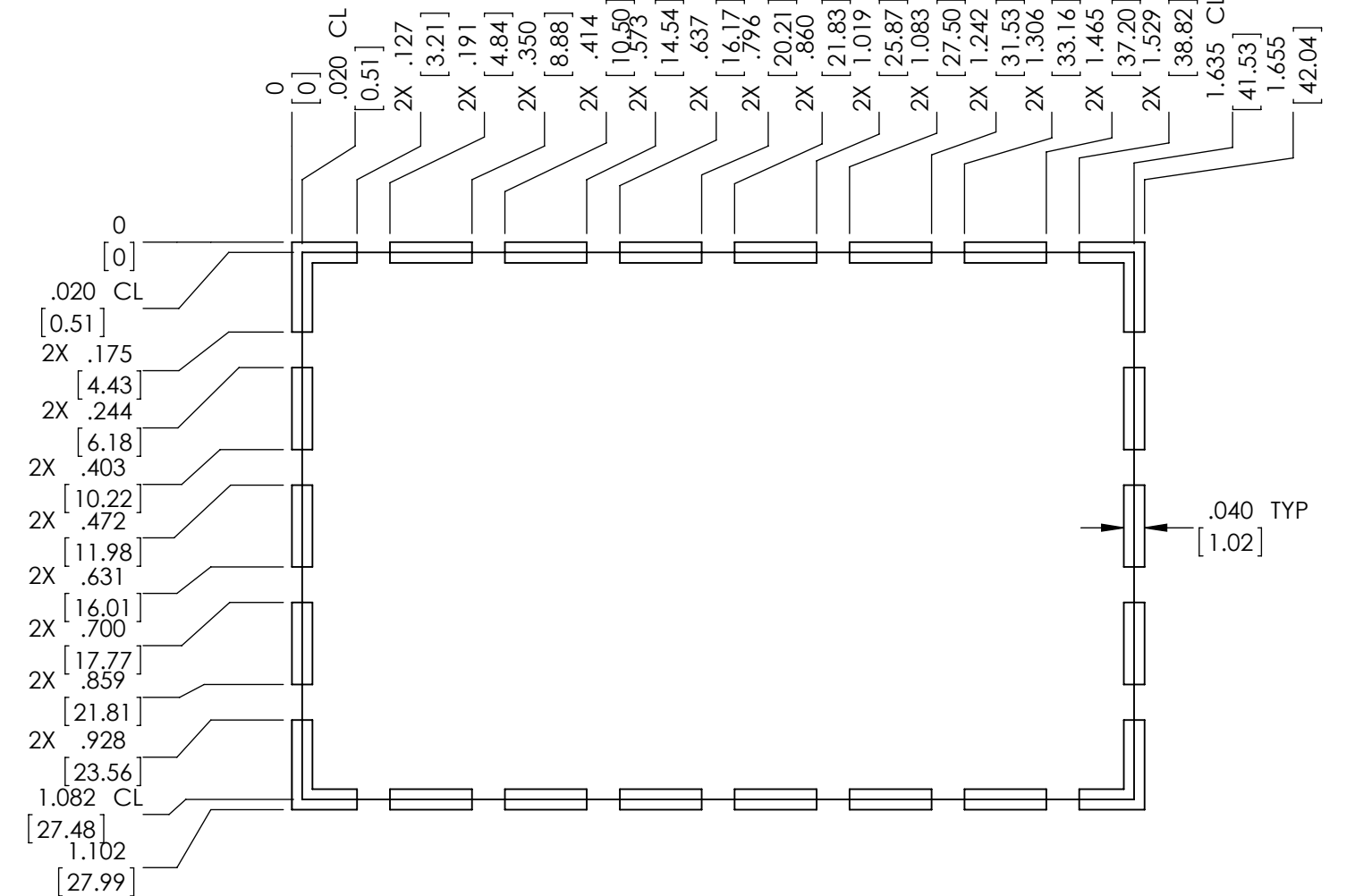
TRACE PATTERN
