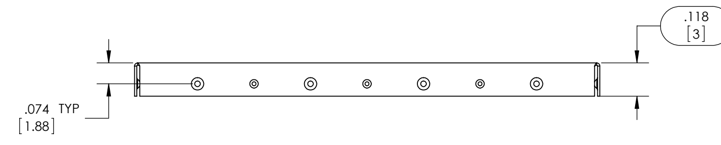
FORMED COVER
