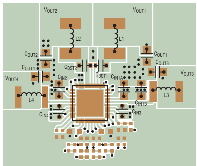
Figure 9. Recommended PCB Layout
