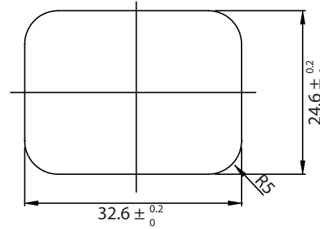
PANEL CUTOUT
