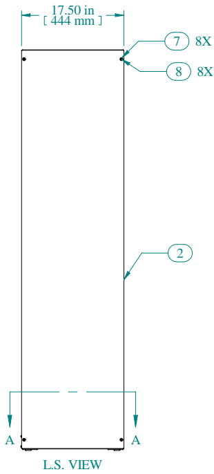
L.S. VIEW
