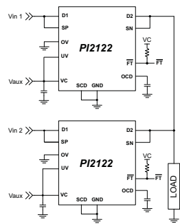
PI2122: High-side Active ORing with Load Disconnect
