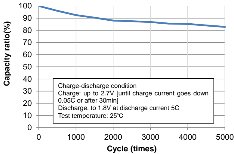
Fig. 42: Capacity ratio (%) of UMAC040130A003TA01 after cycle test at 100mA(Quick charge)
