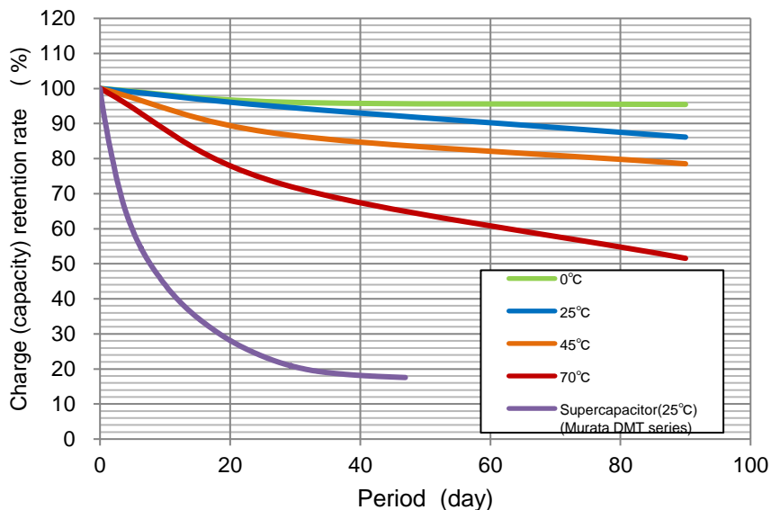
Fig.11 : Charge (capacity) retention rate of UMAC040130A003TA01 exposed at each temperature after full charge
