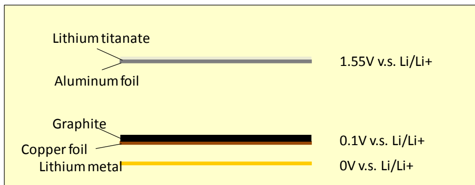
Fig. 25: Negative electrode active material and electrode foil
