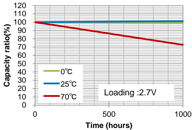
Fig.40: Capacity ratio after applying charge voltage(2.7V) continuously (UMAC040130A003TA01)
