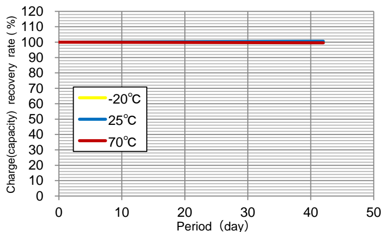
Fig. 39: Charge(capacity) recovery rate(%) (UMAL361421B024TA01)
