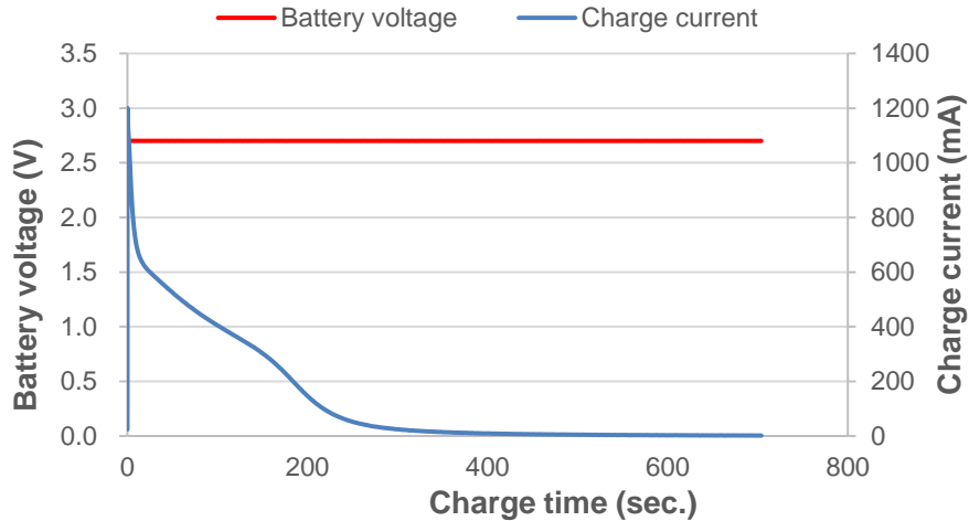
Fig. 27 Charge time, charge voltage and charge current (CV charge of UMAL361421B024TA01)
