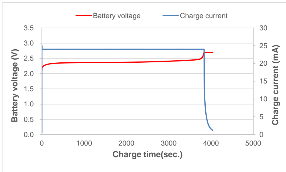
Fig. 26: Charge time, charge voltage and charge current (CC-CV charge of UMAL361421B024TA01)
