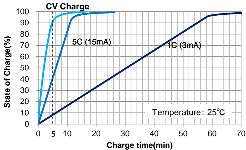
Fig.15: Quick charge at 25°C(UMAC040130A003TA01)
