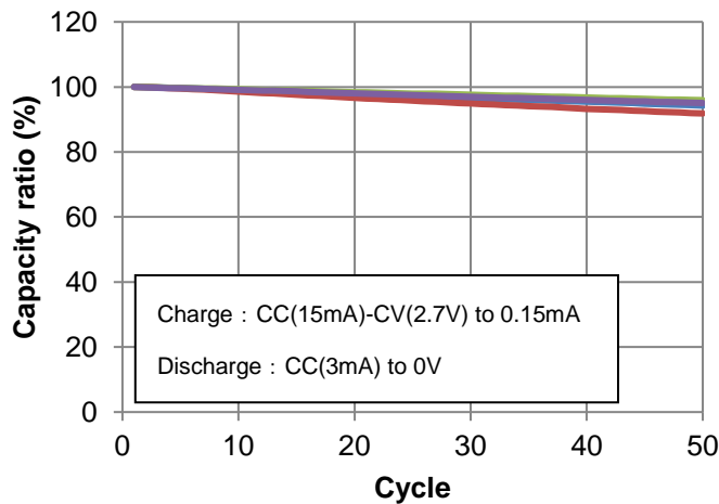
Fig. 24 Capacity ratio (vs. initial value) in the excessive discharge cycle test
