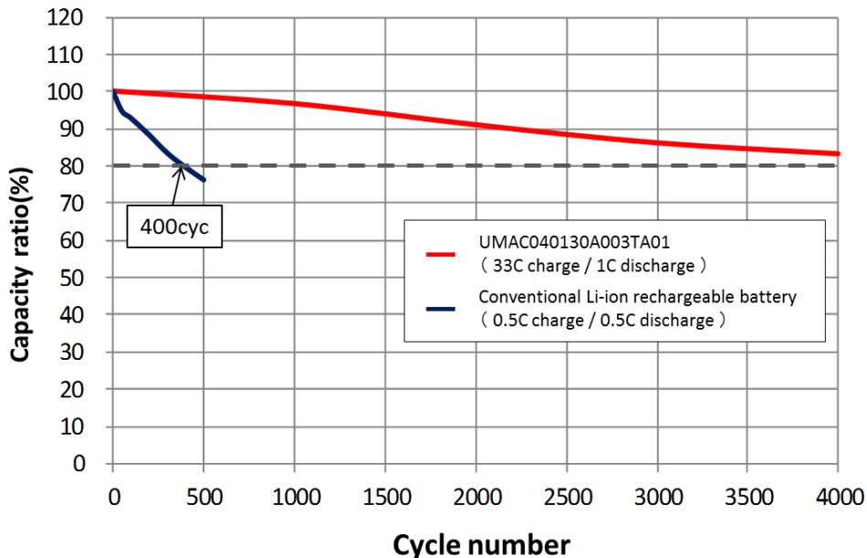
Fig. 17: Charge-discharge cycle characteristic of UMAC040130A003TA01 after repeated quick charge-discharge cycle (Capacity ratio vs. initial value)
