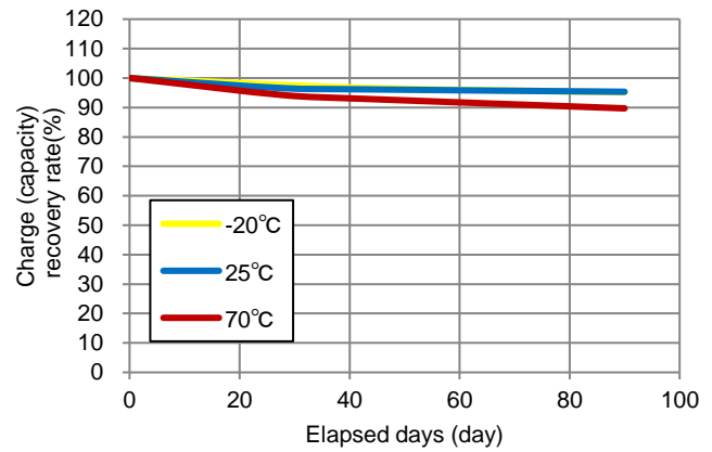
Fig. 37: Charge(capacity) recovery rate (UMAL361421B024TA01)
