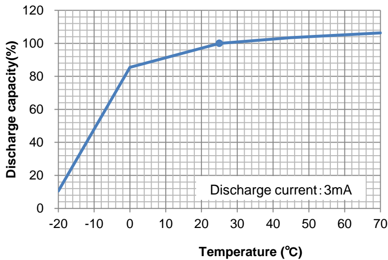
Fig.32: Relationship between temperature and discharge capacity (UMAC040130A003TA01)
