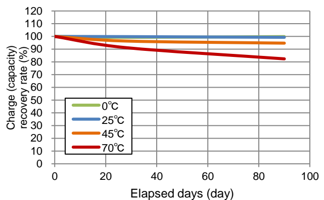
Fig. 35: Charge(capacity) recovery rate (UMAC040130A003TA01)
