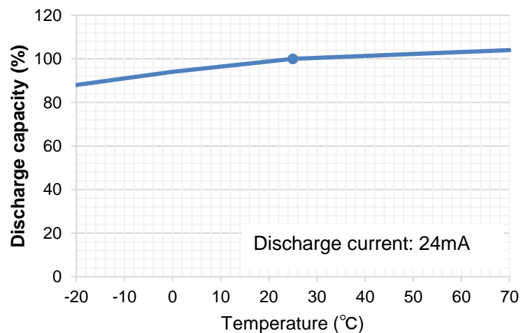
Fig. 33: Relationship between temperature and discharge capacity (UMAL361421B024TA01)
