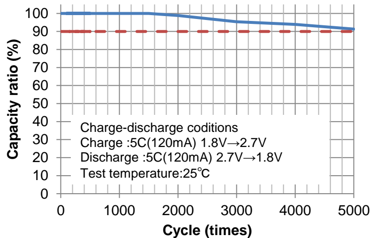
Fig. 43 Capacity ratio of CV charge cycle(%) (UMAL361421B024TA01)
