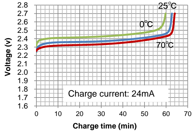
Fig. 21 : Charge curve at 0°C~70°C (UMAL361421B024TA01)
