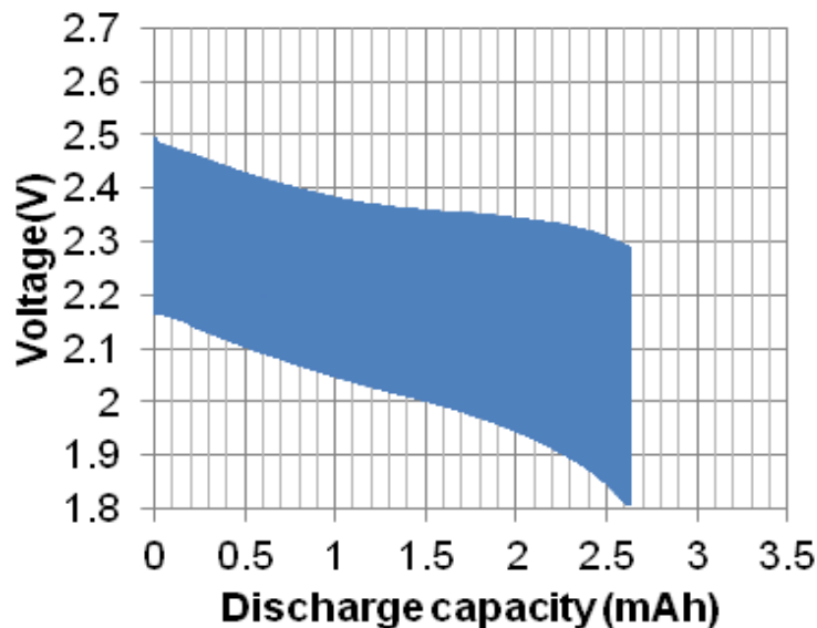
Fig. 23 Pulse discharge by the cycle of (1)30mA, 10msec discharge (2) Rest 15sec. at -20°C (UMAC040130A003TA01)
