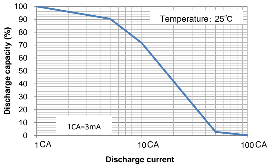
Fig. 29: Relationship between discharge current and discharge capacity (UMAC040130A003TA01)
