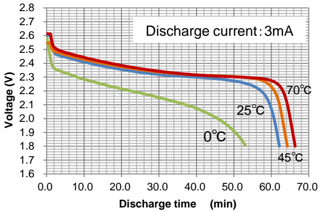
Fig. 18: Discharge curve at 0°C~70°C (UMAC040130A003TA01)
