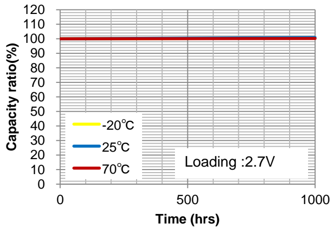
Fig. 41 Capacity ratio after applying charge voltage(2.7V) continuously (UMAL361421B024TA01)
