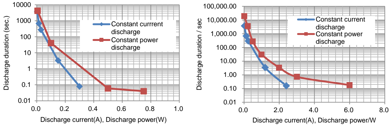
Fig. 9: Discharge current(A), discharge power(W), and discharge time(sec.) (Left: UMAC040130A003TA01, Right: UMAL361421B024TA01)
