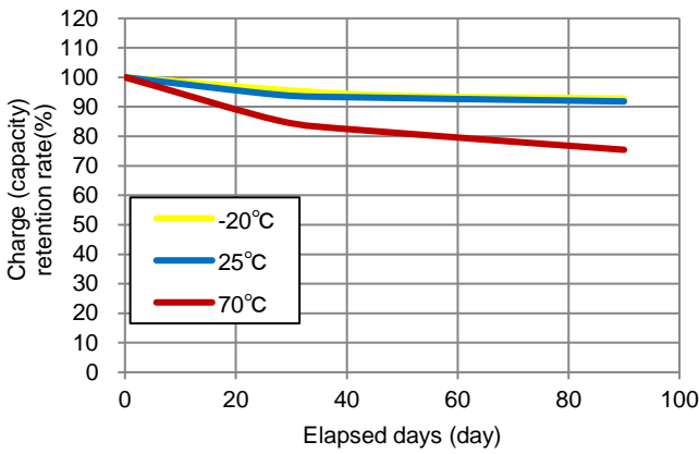
Fig. 36: Charge(capacity) retention rate (UMAL361421B024TA01)
