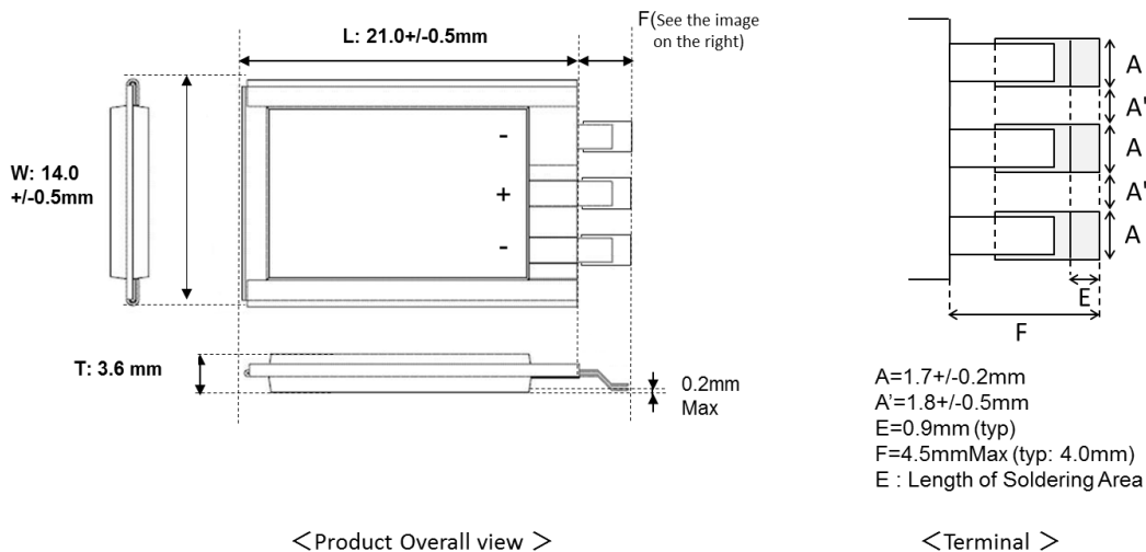
Fig. 7: Shape and dimension (UMAL361421B024TA01)
