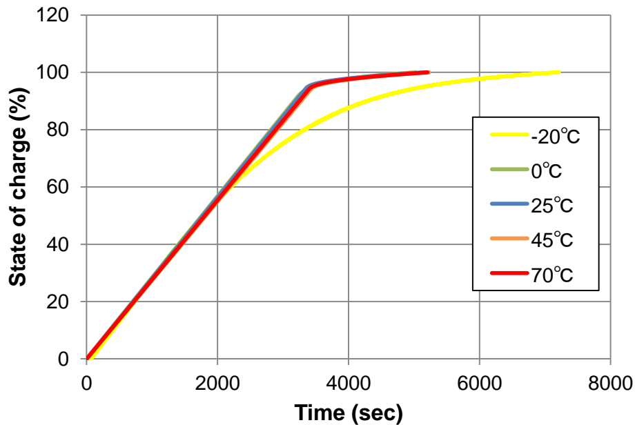
Fig.31: Relationship between temperature and charge capacity (UMAC040130A003TA01)
