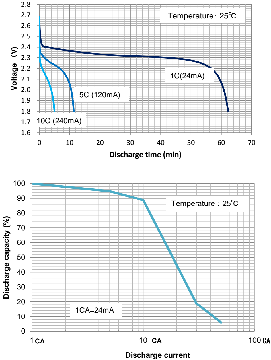
Fig. 30: Relationship between discharge current and discharge capacity (UMAL361421B024TA01)
