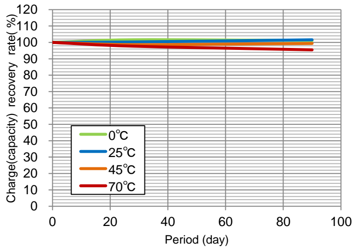
Fig.38: Charge(capacity) recovery rate(%) (UMAC040130A003TA01)
