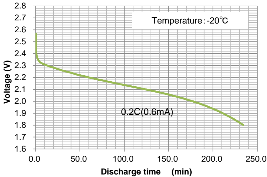
Fig. 22 Discharge curve at -20°C (UMAC040130A003TA01)
