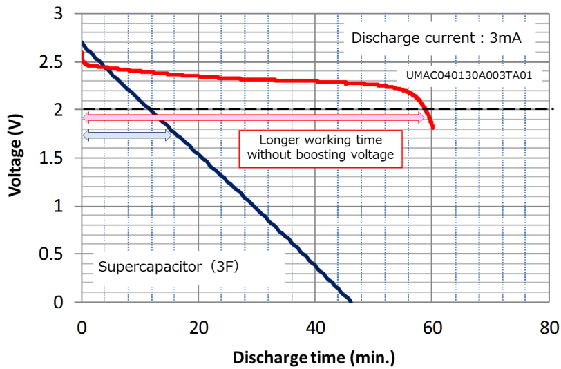
Fig.13: Discharge curves of UMAC and supercapacitor(capacitance:3F)
