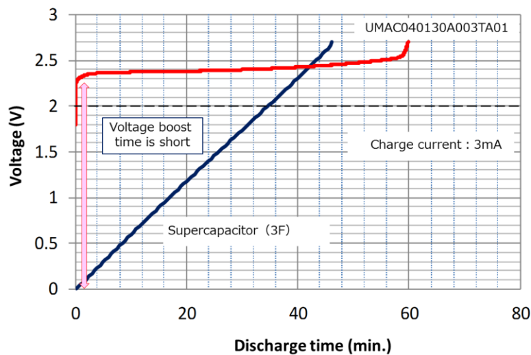
Fig.14: Charge curves of UMAC040130A003TA01 and supercapacitor (capacitance: 3F)
