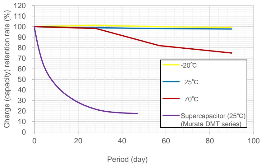
Fig.12 : Charge (capacity) retention rate of UMAC040130A003TA01 exposed at each temperature after full charge
