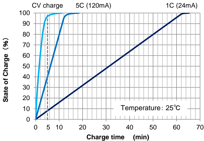
Fig.16: Quick charge at 25°C(UMAL361421B024TA01)
