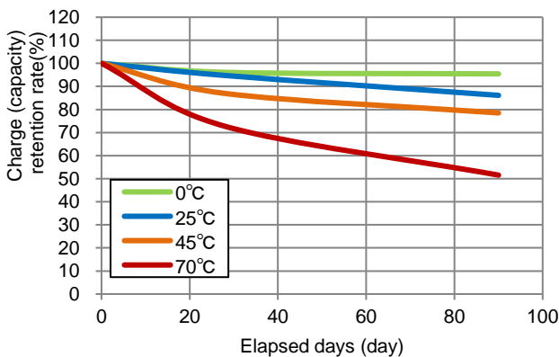
Fig. 34: Charge(capacity) retention rate (UMAC040130A003TA01)
