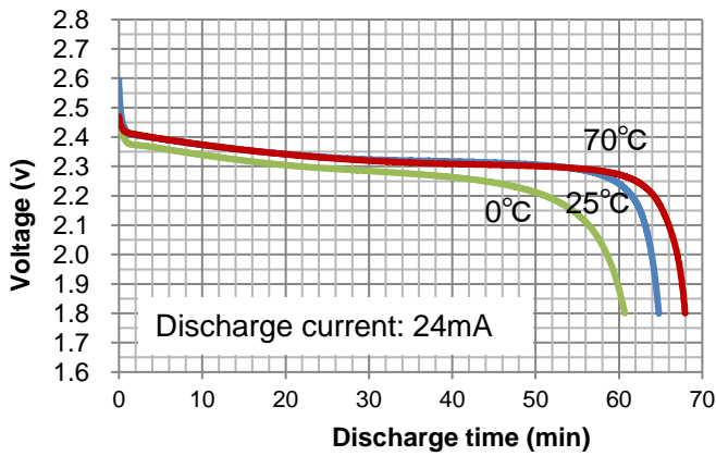
Fig. 20: Discharge curve at 0°C~70°C (UMAL361421B024TA01)
