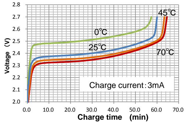
Fig. 19: Charge curve at 0°C~70°C (UMAC040130A003TA01)
