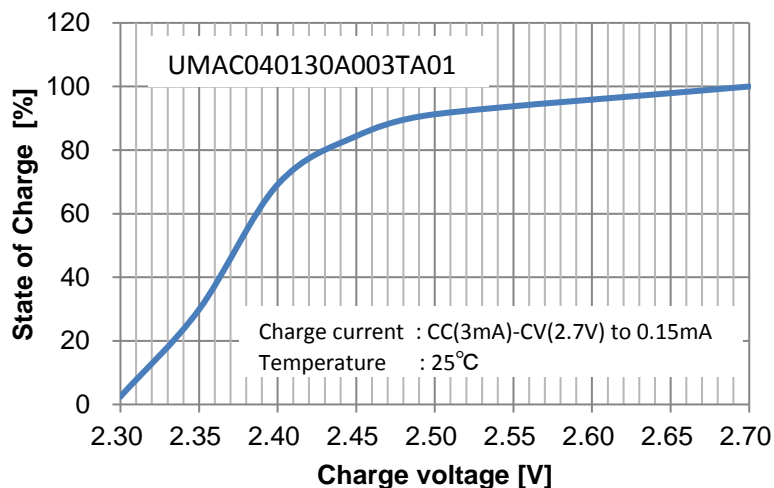
Fig. 28 Charge voltage and state of charge (UMAC040130A003TA01)
