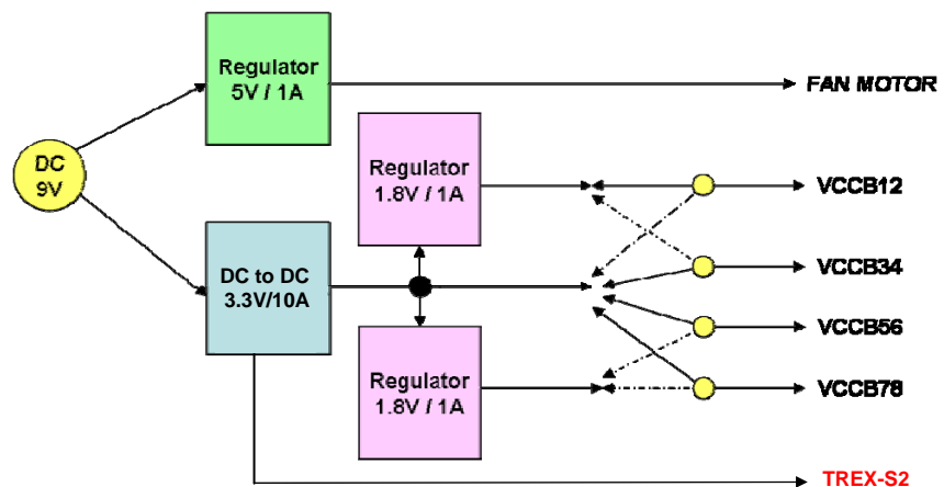
Figure 3.1 The Bank Voltage Selection Scheme
