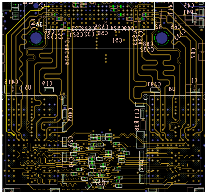
Figure 12. i.MX 8MDQLQ validation board DDR4 routing (Layer 6)
