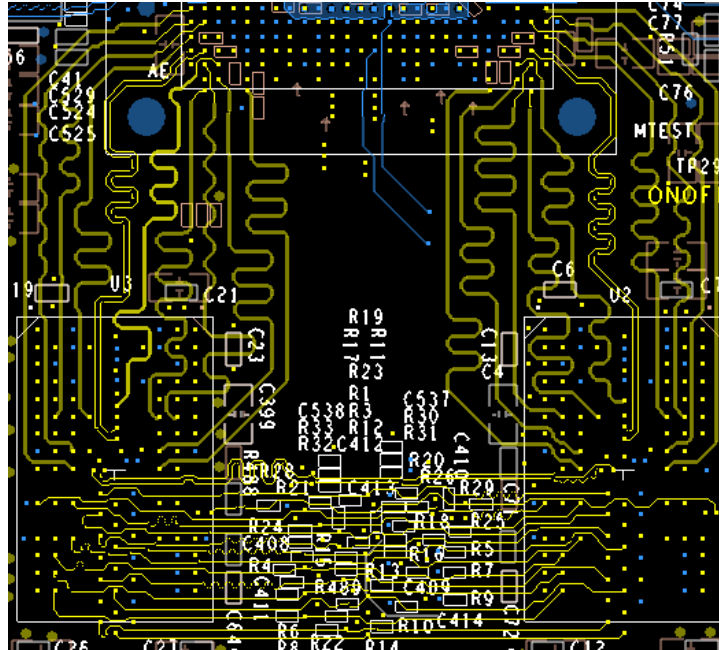
Figure 15. i.MX 8MDQLQ validation board DDR3L routing (Layer 3)
