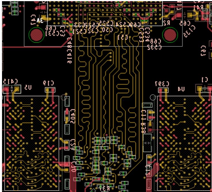
Figure 13. i.MX 8MDQLQ validation board DDR4 routing (Layer 8)
