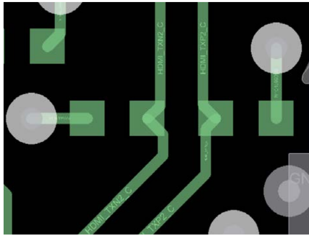
Figure 25. HDMI interface pull-down resistor placement
