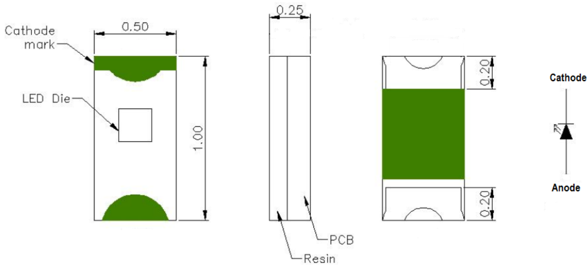
Figure 1: Package Dimensions
