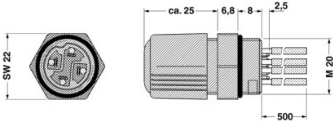
Dimensioned drawing
