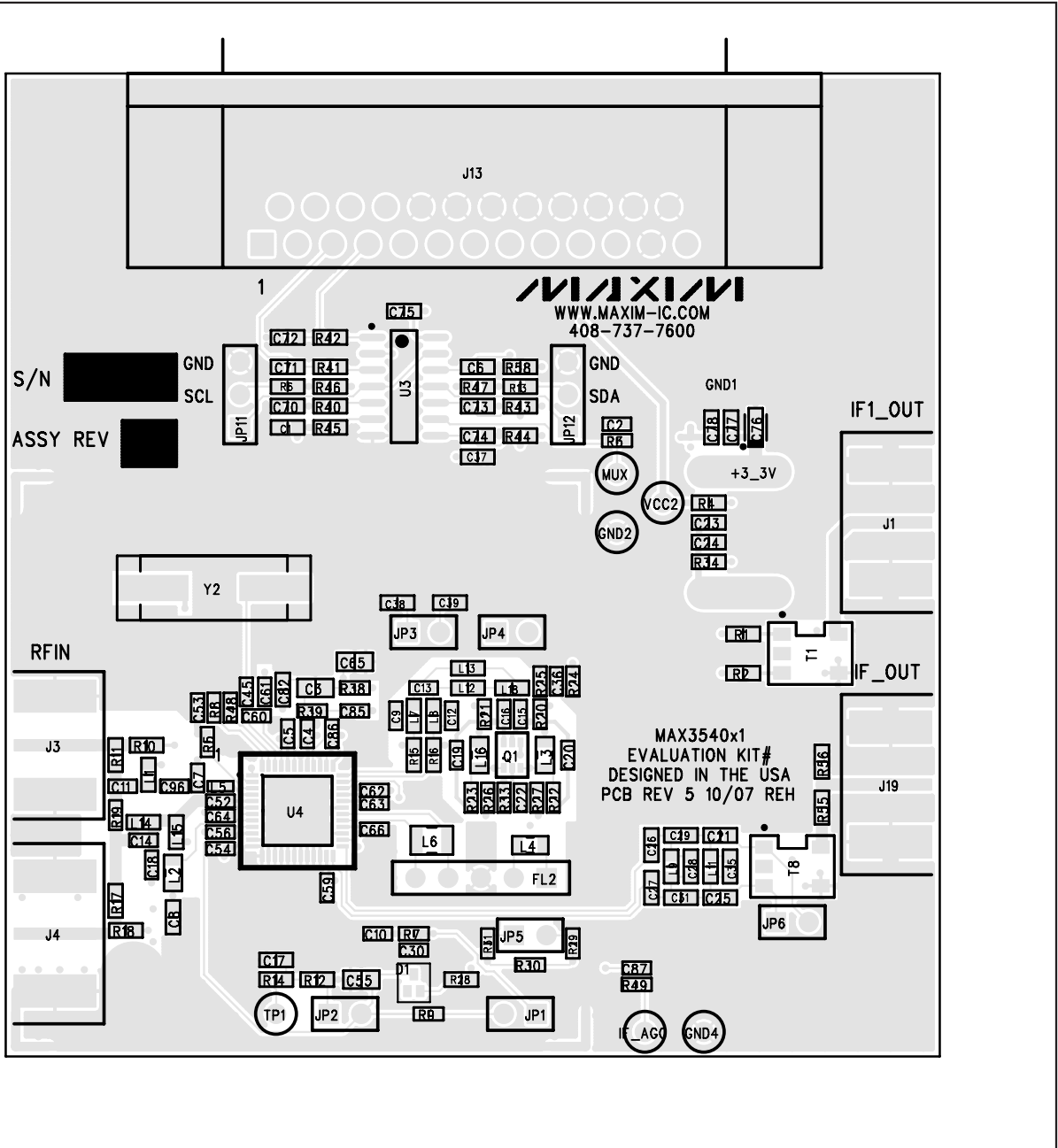
Figure 2. MAX3540 EV Kit PCB Layout—Component Placement Guide
