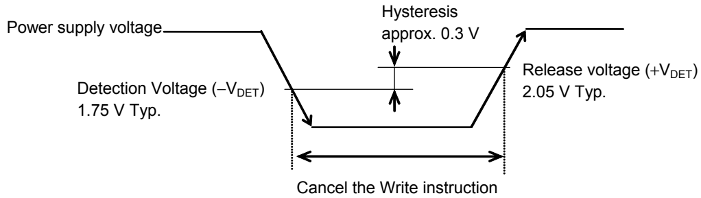
Figure 27 Operation during Low Power Voltage
