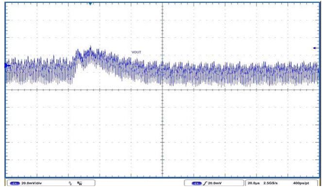
FIGURE 19. LOAD TRANSIENT (50A TO 0A STEP, SLEW_RATE = 2.5A/µs)
