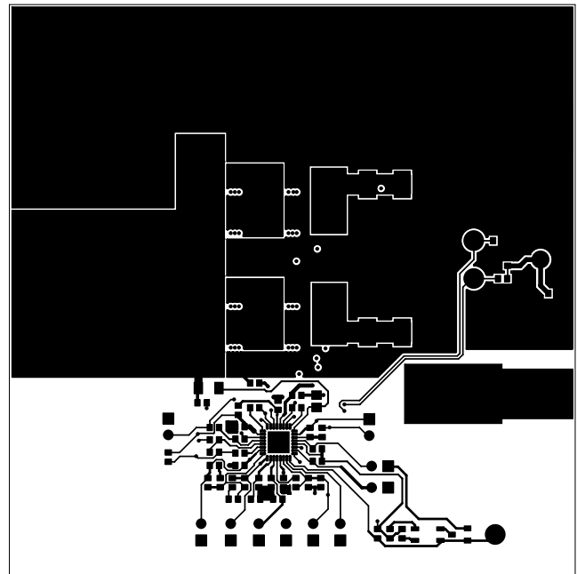
FIGURE 4. TOP LAYER
