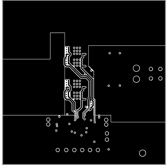
FIGURE 6. 3 rd LAYER
