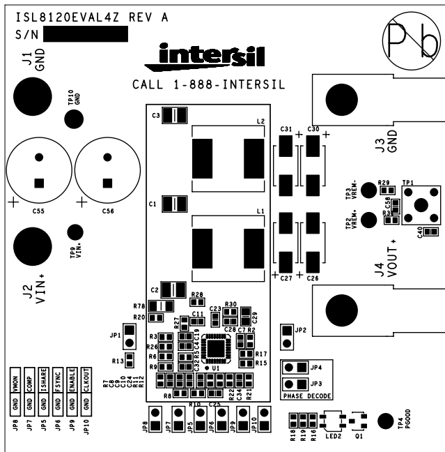
FIGURE 3. TOP SILKSCREEN
