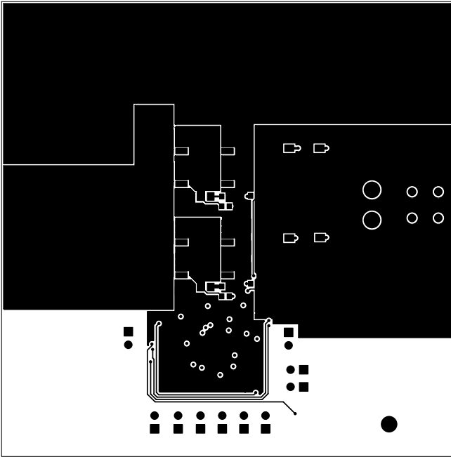
FIGURE 9. BOTTOM LAYER
