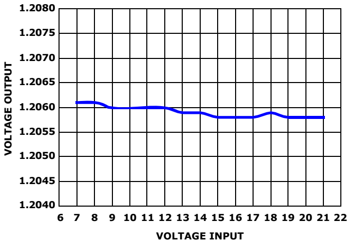
FIGURE 14. LINE REGULATION
