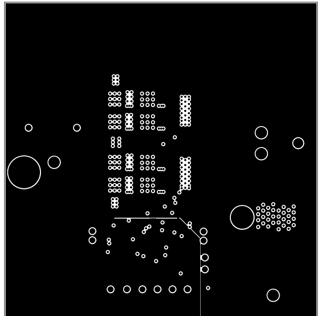
FIGURE 8. 5 th LAYER
