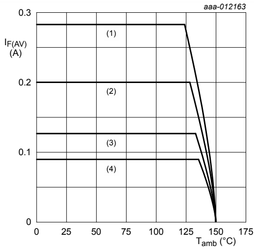
FR4 PCB, mounting pad for anode and cathode 1 cm 2 each T j = 150 °C (1) δ = 1; DC (2) δ = 0.5; f = 20 kHz (3) δ = 0.2; f = 20 kHz (4) δ = 0.1; f = 20 kHz
