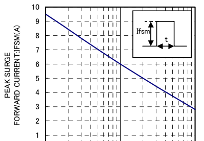
IFSM-t CHARACTERISTICS
