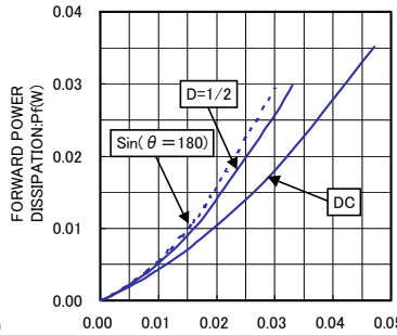
Io-Pf CHARACTERISTICS
