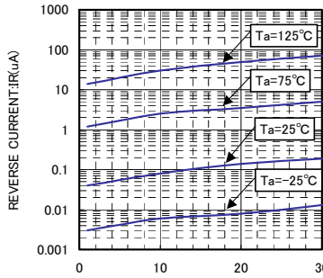
VR-IR CHARACTERISTICS
