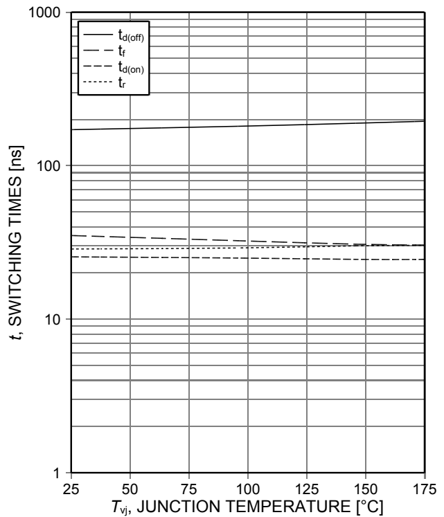
Figure 10. Typical switching times as a function of junction temperature (inductive load, V_{CE}=400\text{V} , V_{GE}=0/15\text{V} , I_C=50\text{A} , R_{G(on)}=12\Omega , R_{G(off)}=12\Omega , dynamic test circuit in Figure E)
