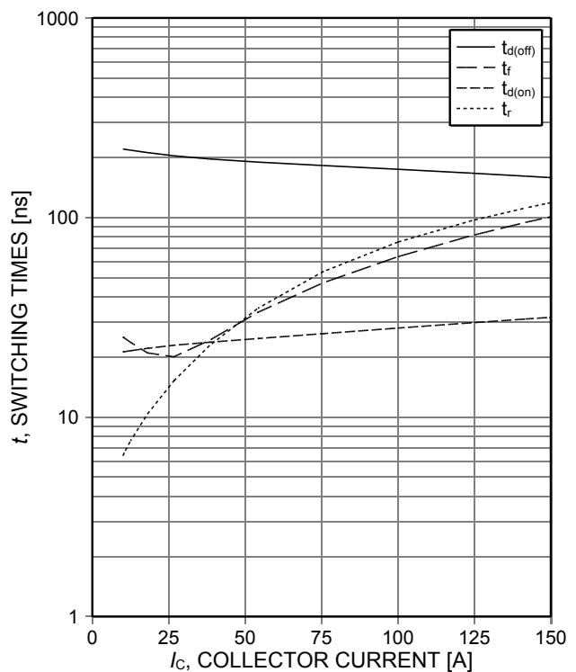
Figure 8. Typical switching times as a function of collector current (inductive load, T_{vj}=150^{\circ}\text{C} , V_{CE}=400\text{V} , V_{GE}=0/15\text{V} , R_{G(on)}=12\Omega , R_{G(off)}=12\Omega , dynamic test circuit in Figure E)
