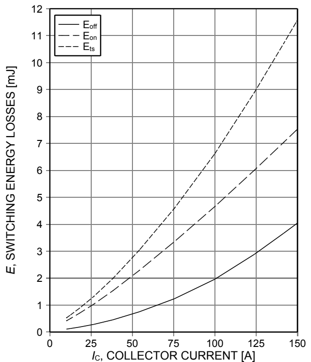
Figure 12. Typical switching energy losses as a function of collector current (inductive load, T_{vj}=150^{\circ}\text{C} , V_{CE}=400\text{V} , V_{GE}=0/15\text{V} , R_{G(on)}=12\Omega , R_{G(off)}=12\Omega , dynamic test circuit in Figure E)
