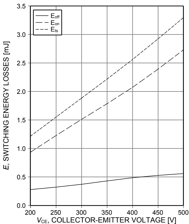
Figure 15. Typical switching energy losses as a function of collector emitter voltage (inductive load, T_{vj}=150^{\circ}\text{C} , V_{GE}=0/15\text{V} , I_C=50\text{A} , R_{G(on)}=12\Omega , R_{G(off)}=12\Omega , dynamic test circuit in Figure E)
