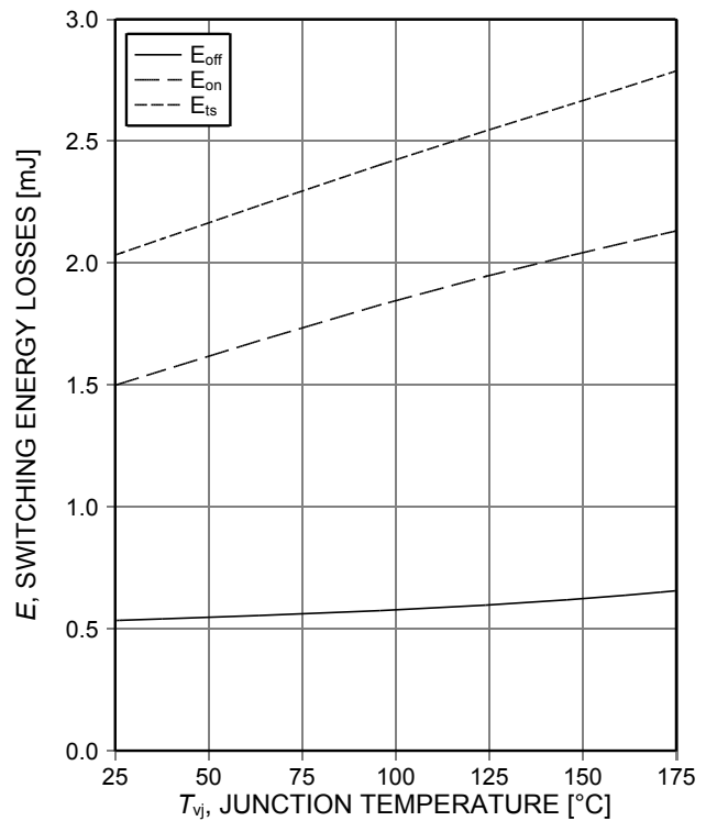
Figure 14. Typical switching energy losses as a function of junction temperature (inductive load, V_{CE}=400\text{V} , V_{GE}=0/15\text{V} , I_C=50\text{A} , R_{G(on)}=12\Omega , R_{G(off)}=12\Omega , dynamic test circuit in Figure E)
