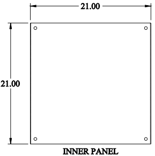
INNER PANEL
