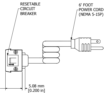
ASSEMBLY - VIEW FROM END
