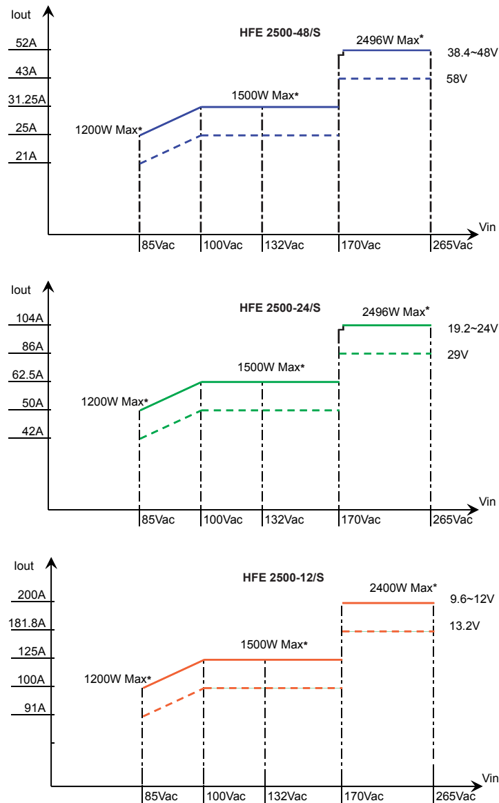
Fig-1 HFE2500 rated output Current and Voltage versus Line Voltage.
