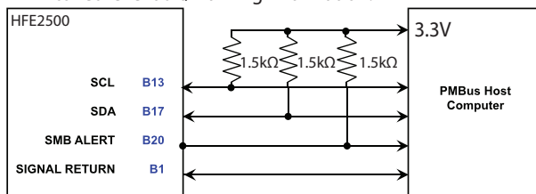
Fig-3.6 PMBus Typical connection
