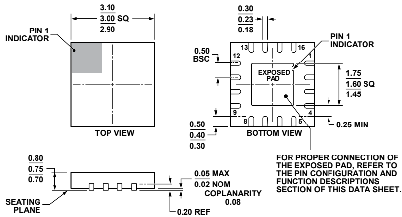
Figure 55. 16-Lead Lead Frame Chip Scale Package [LFCSP] 3 mm × 3 mm Body and 0.75 mm Package Height (CP-16-22)
