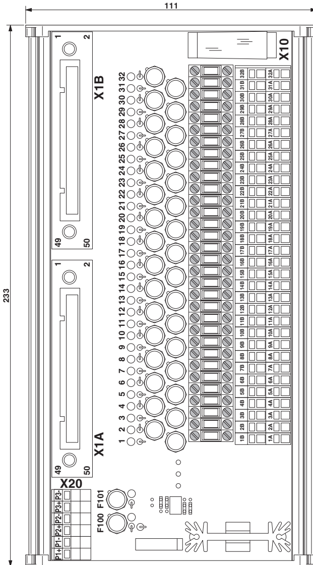
Dimensional drawing
