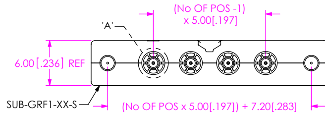
FIG 1 GRFX-P-C-04-XXXX-CXX-S-S-XX SHOWN
