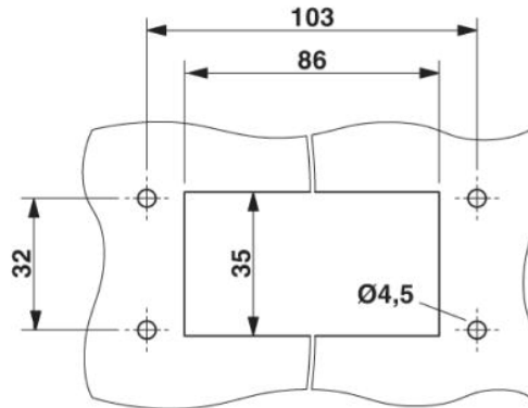
Panel cutout
