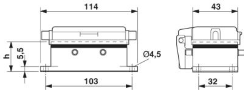
Dimensional drawing
