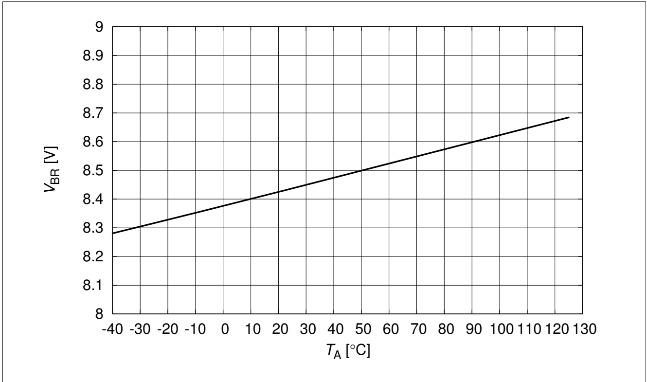
Figure 4-3 Reverse voltage: V_{BR} = f(T_A) , I_R = 1 \text{ mA}
