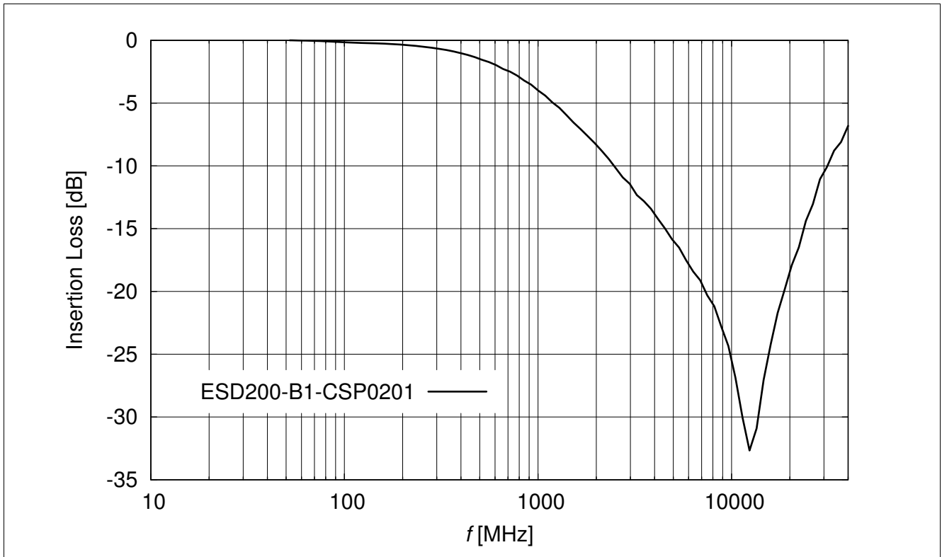
Figure 4-11 Insertion loss vs. frequency in a 50 \Omega system
