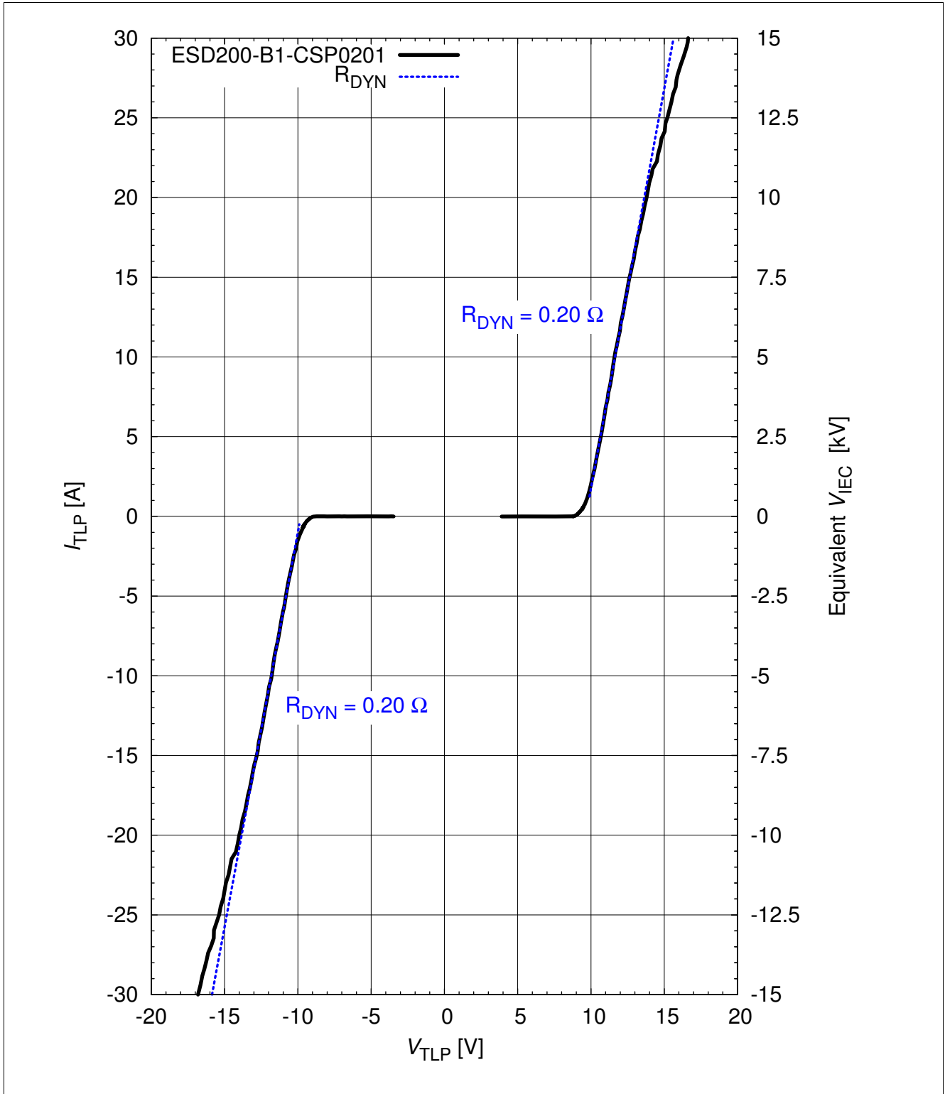
Figure 4-9 Clamping voltage (TLP): I_{TLP} = f(V_{TLP}) [1]
