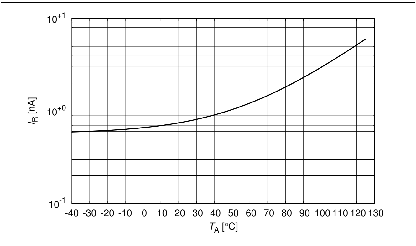
Figure 4-2 Reverse current: I_R = f(T_A) , V_R = 5.5\text{ V}
