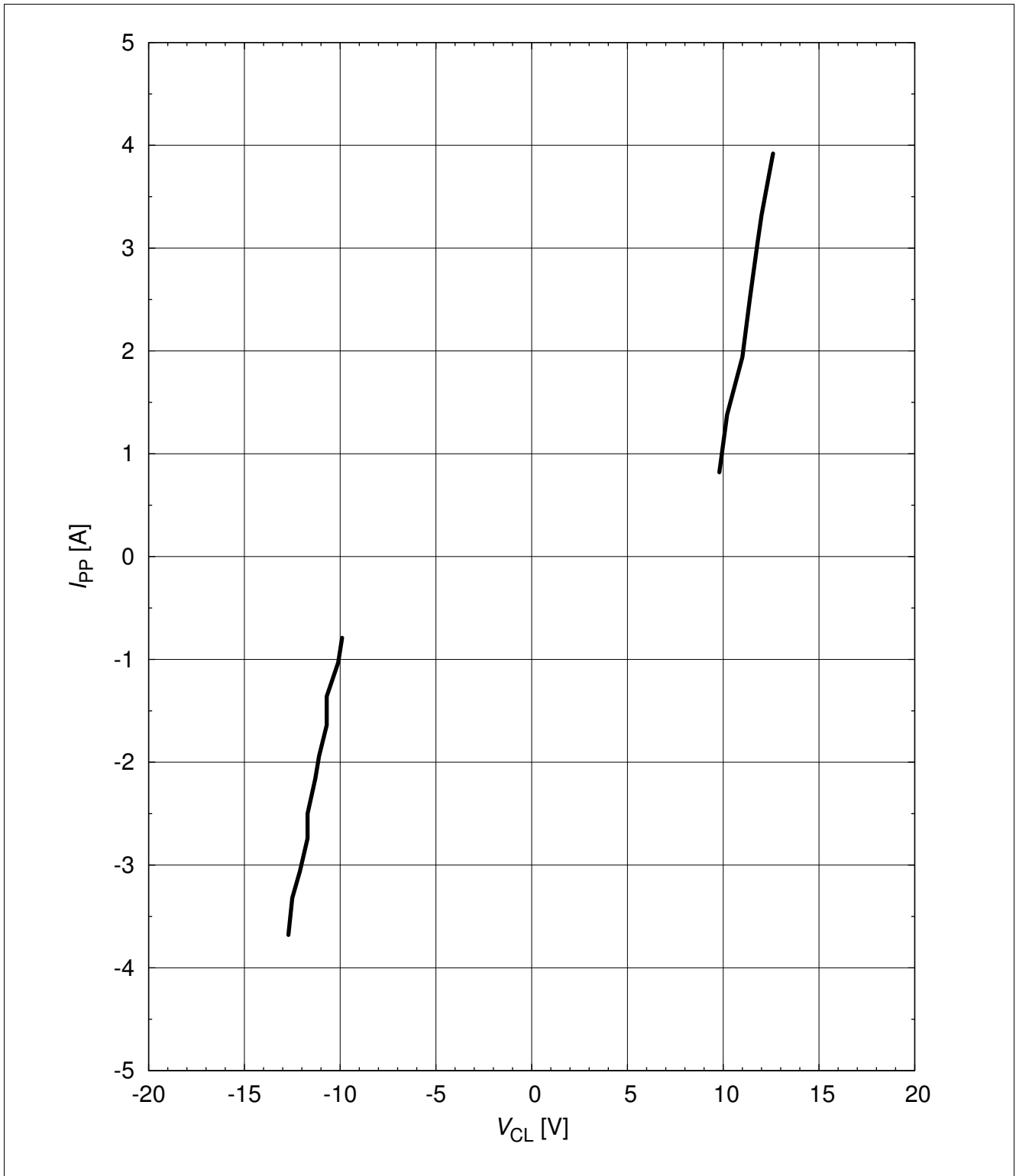
Figure 4-10 Clamping voltage (Surge): I_{PP} = f(V_{CL}) [1]
