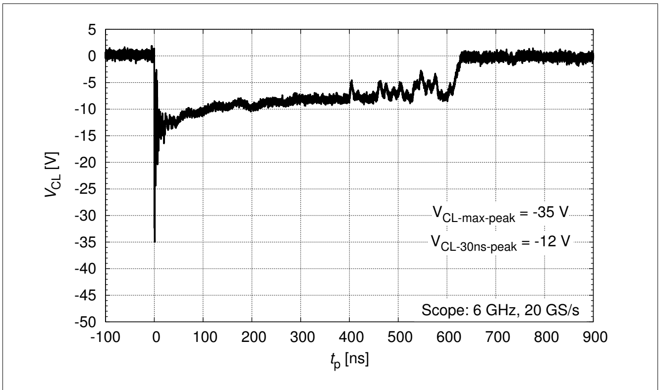
Figure 4-8 Clamping voltage (ESD): V_{CL} = f(t) , 15 kV negative pulse
