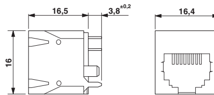
Dimensioned drawing
