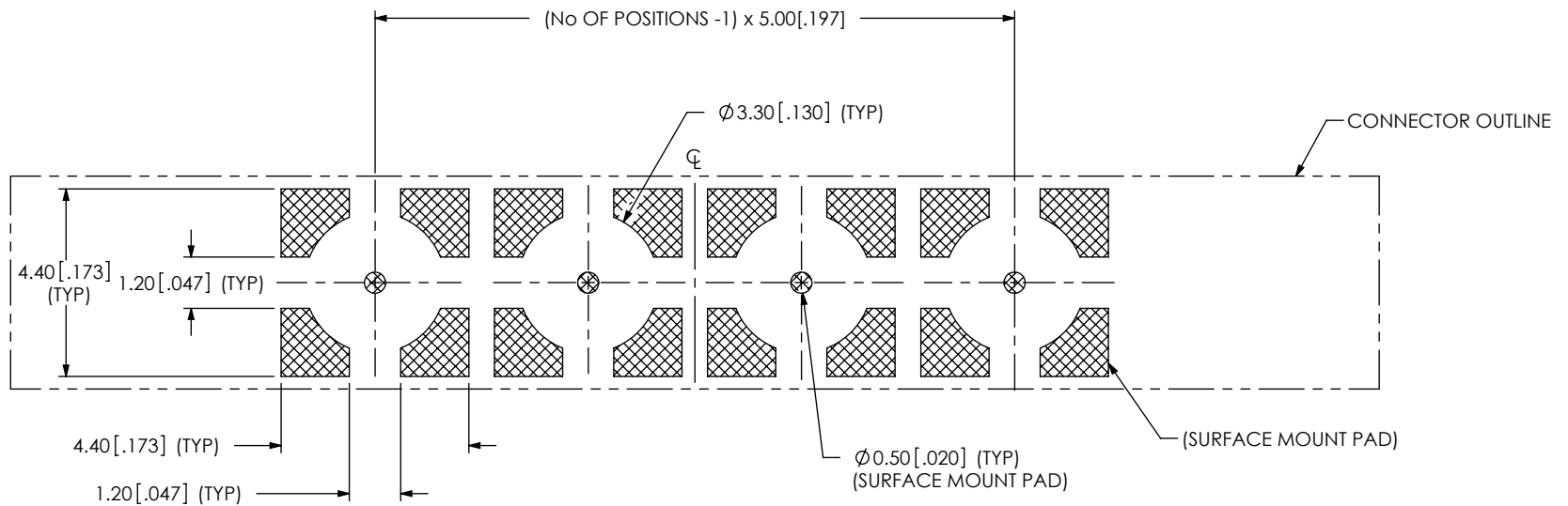
FIG 4 FOOTPRINT FOR GRF7-J-P-04-XX-ST-SM1-X SHOWN (SAME AS FIG 1 EXCEPT AS NOTED)
