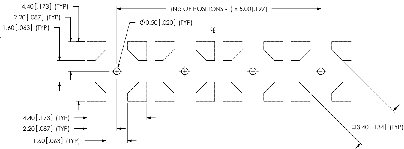
FIG 3 STENCIL FOR GRF7-J-P-04-XX-ST-MT1 SHOWN (SEE NOTE 1, SHT 3)
