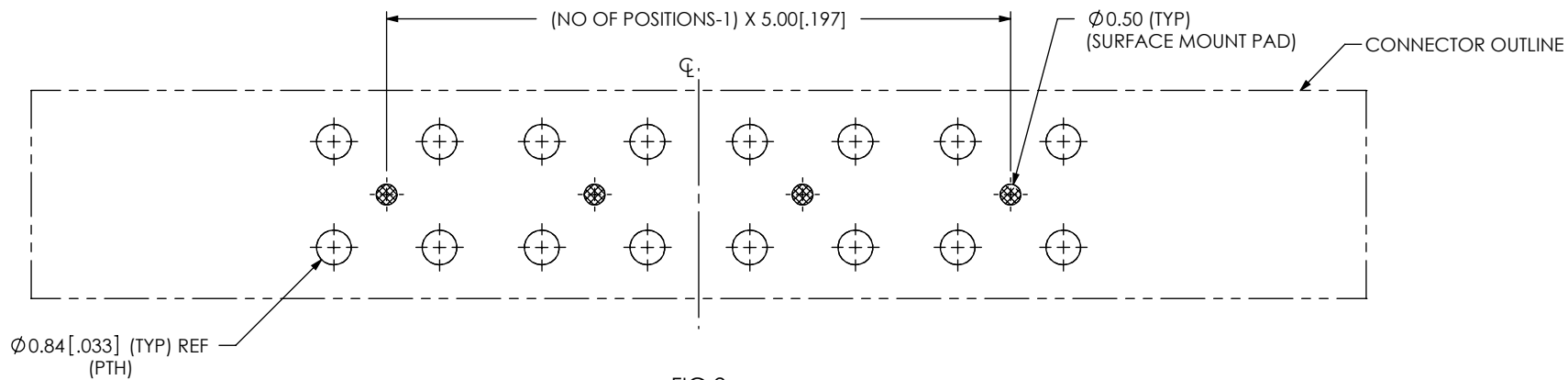
FIG 2 FOOTPRINT FOR GRF7-J-P-04-XX-ST-MT1-X SHOWN (SAME AS FIG 1 EXCEPT AS NOTED)
