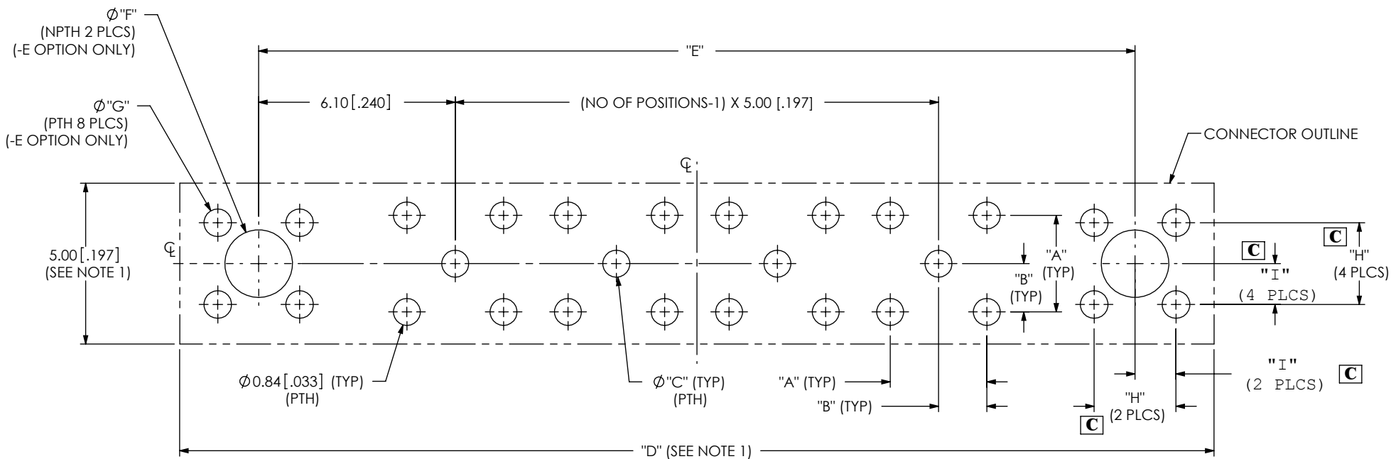
FIG 1 FOOTPRINT FOR GRFX-J-P-04-XX-ST-TH1-X SHOWN
