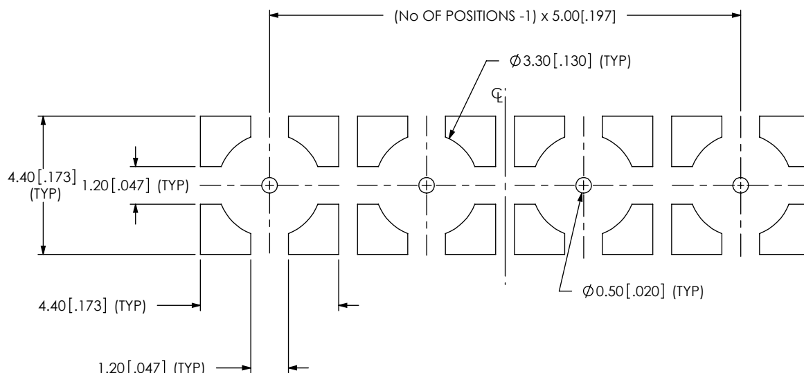
FIG 5 STENCIL FOR GRF7-J-P-04-XX-ST-SM1 SHOWN (SAME AS FIG 4 EXCEPT AS NOTED) (SEE NOTE 1, SHT 5)
