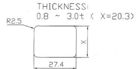
PANEL CUT-OUT
