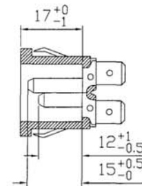
SECTION. AL
